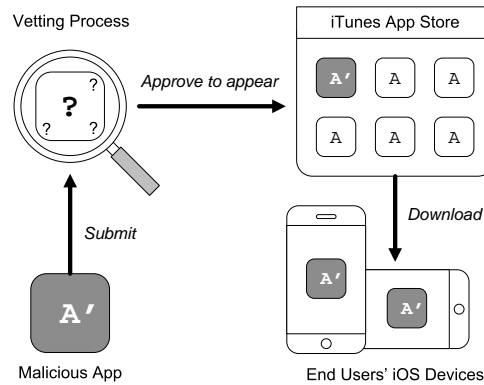
Fig. 1. Threat model.
